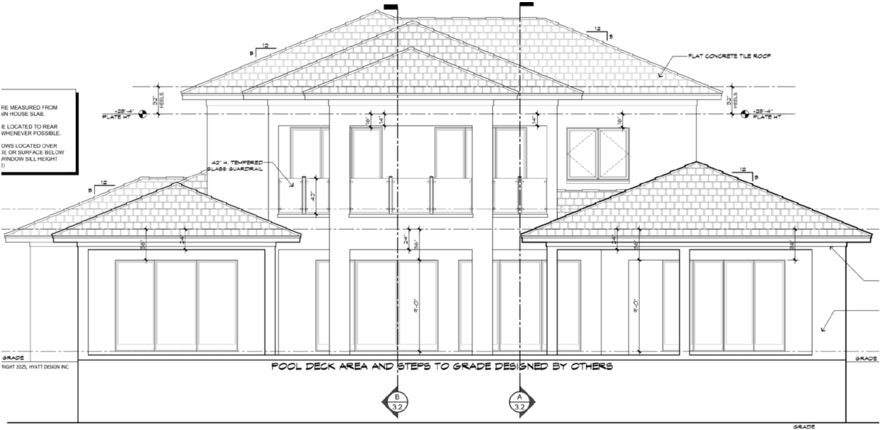
Rear Elevation
